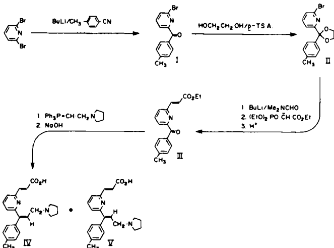
Scheme 1—Preparation of triprolidine hapten derivative.
